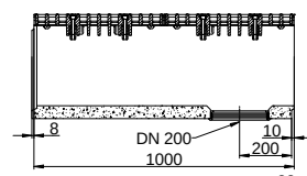
Vertical outlet
