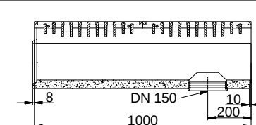
Vertical outlet
