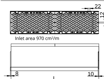
Basic element
