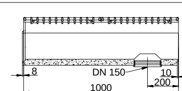
Vertical outlet
