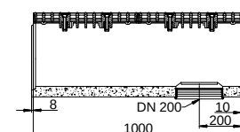
Vertical outlet
