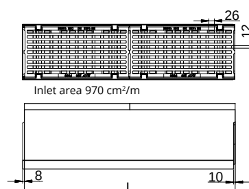
Basic element
