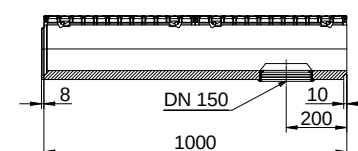
Vertical outlet
