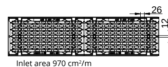
Basic element
