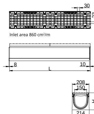
Vertical outlet
