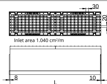
Basic element
