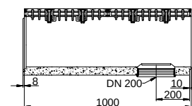
Vertical outlet
