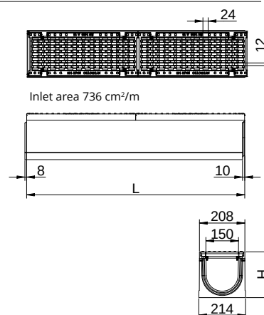
Vertical outlet
